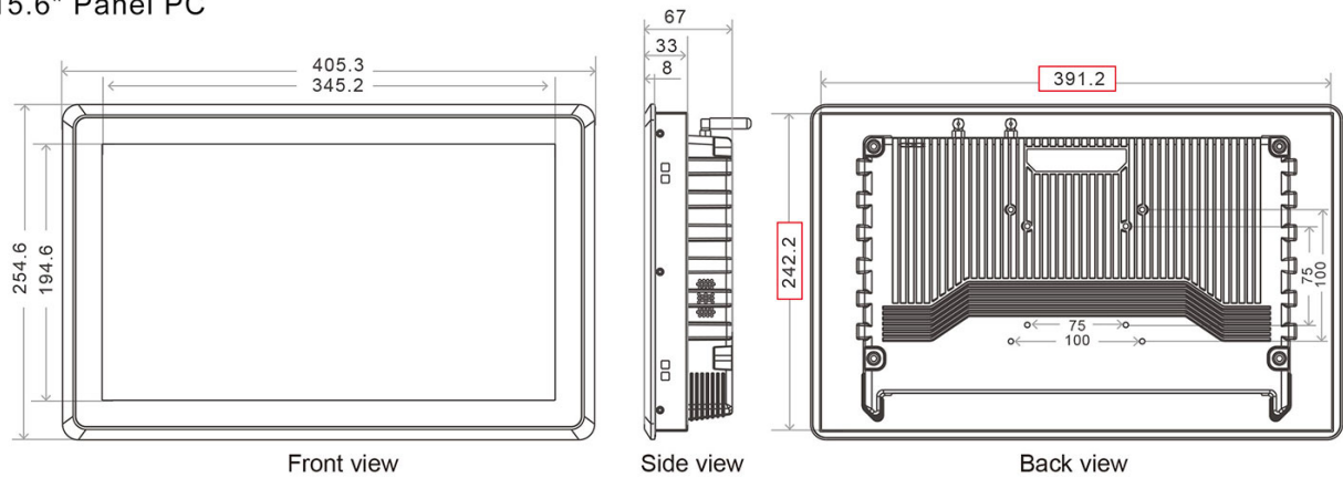
15.6" Panel PC
